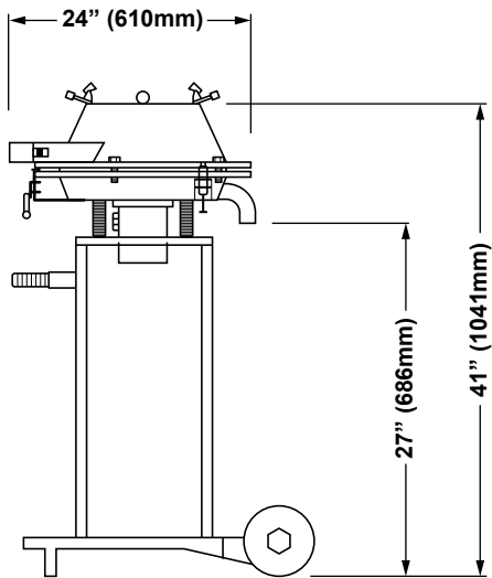
SCREENER 450 24" (609.6mm) DIAMETER
