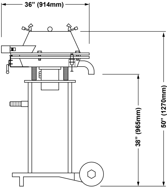
SCREENER 600 36" (914.4mm) DIAMETER
